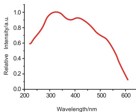
激发光谱 EX Spectrum
